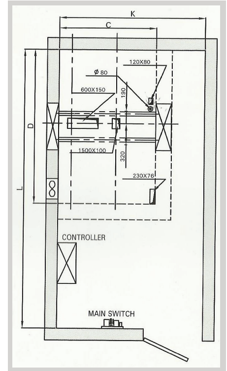
MACHINE ROOM PLAN
